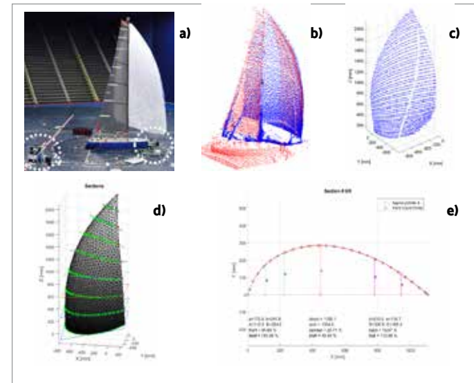
2. Wind tunnel test: experimental setup (a), point cloud registration (b), sail cluster extraction (c), surface reconstruction and sections (d), computed sail geometrical parameters (e).
