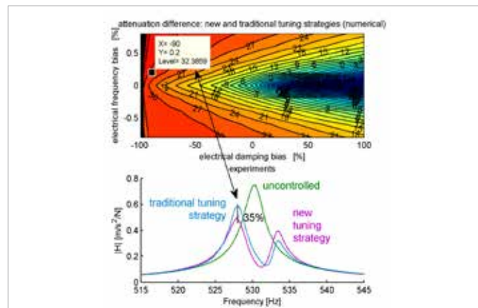
1. New LR tuning strategy: robustness comparison and validation
