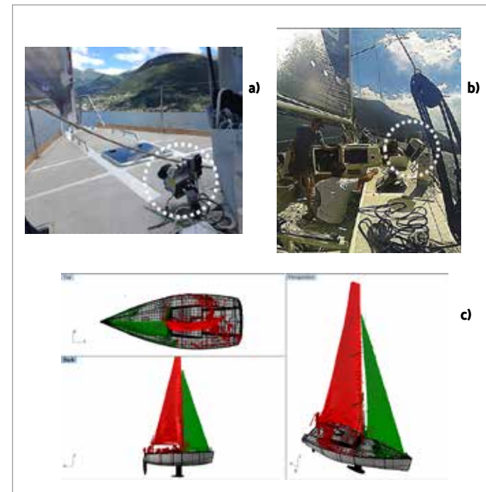
3. Full scale test: experimental setup (a-b), reconstruction of the sail plan for a close-hauled case (c).
