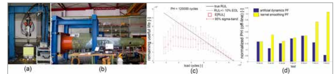
1. Aeronautical panels subject to tension-tension fatigue (a) and a real helicopter tail (b) have been used as case studies. The algorithm is able to predict the RUL of the structure many cycles before the true failure (c), and its performance has been assessed using metrics like the prognostic horizon (d).
