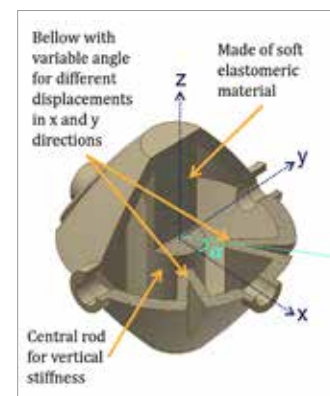
1. Concept of the soft biaxial actuator
