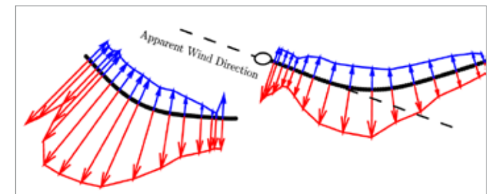
3. Example of measured pressure distributions over measured flying shapes.
