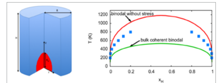
3. Sketch of the geometry for the finite element simulations of the continuum field model. The entire sample has a cylindrical shape; all surfaces, top, bottom and mantle are stress free. A hydride is nucleated near the lower surface, shown here in red. The system has a cylindrical symmetry, which allows to reduce the problem to a two-dimensional description (right). The phase diagram with the coherent surface binodal, obtained from the continuum field model (blue data points). The focus is here on the low temperature data (left).
