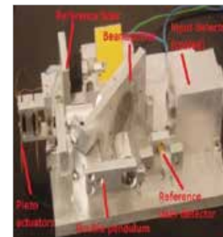
2. The microMIMA interferometer mock-up
