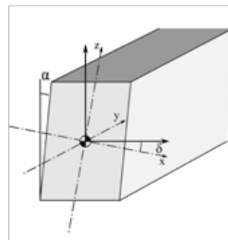
1. A microfabricated elastic element in which the wall angle defect causes a rotation of the principal axes of inertia in the beam section.
