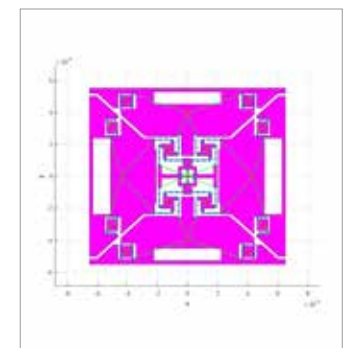
3. Layout of 3-axis gyroscope with low quadrature analyzed with feMEMS approach.
