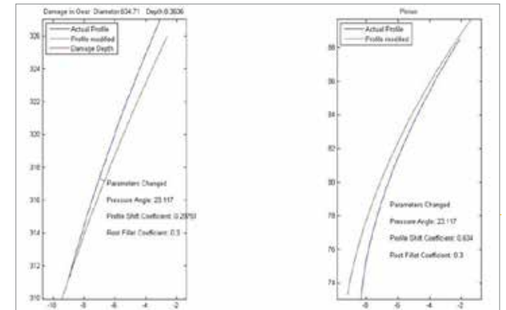
2. Modification chart
