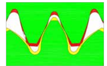
3. Comparative chart of the actual pair and the modified pair. Red area is the stock removal and the yellow area is the amount increased
