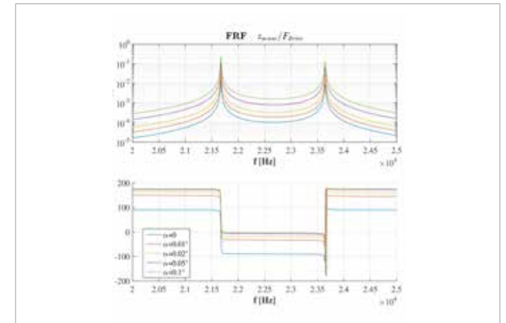
2. Frequency response function of a Coriolis Vibratory Gyroscope along sense direction: quadrature causes an increasing ZRO value at different values of wall angle.
