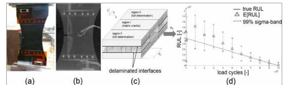
2. Notched cross-ply carbon FRP under tension-tension fatigue (a), X-ray images showing matrix cracks and delamination (b), modeling approach for the estimation of G (c) and RUL prediction using PF (d).
