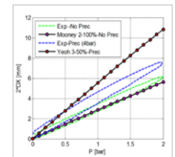
3. Validation of the actuator, with and without preconditioning
