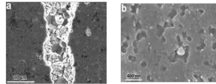
1. SEM micrograph of (a) non-ECAP and (b) UFG ZK60 Mg alloy immersed in PBS solution.
