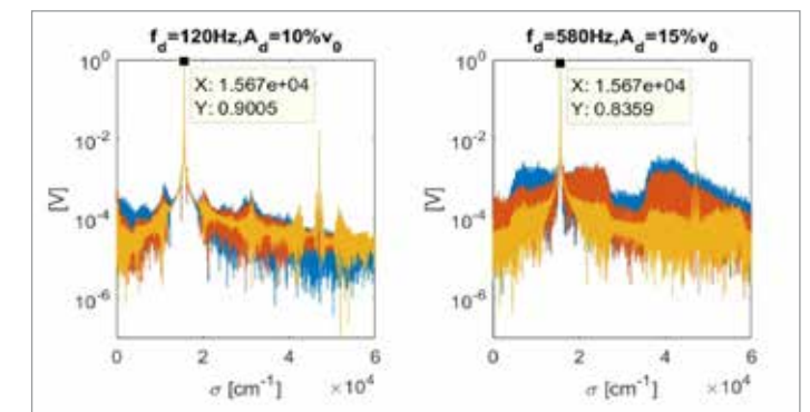
3. Spectrum of the measured reference laser for different disturbance and amplitude frequency computed with Campbell (blue), Hilbert (red) and arccosine (yellow) method
