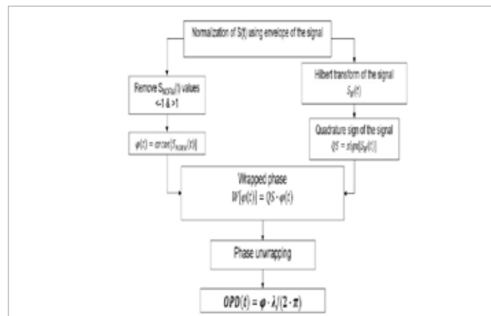
1. Scheme of the arccosine method
